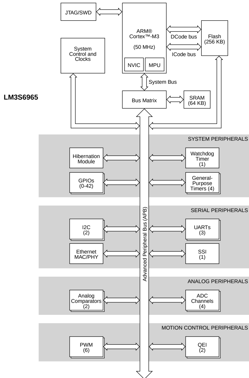
Figure 1-1. Stellaris® LM3S6965 Microcontroller High-Level Block Diagram
